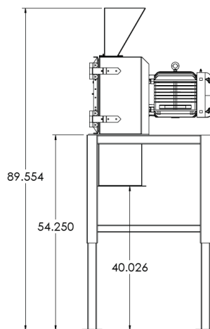
*Shown with 10HP Motor; Legs Fully Extended
