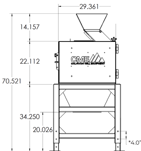
*4.0" Leg Adjustment Increment
